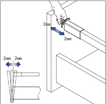
Turn insert to adjust length of rail
