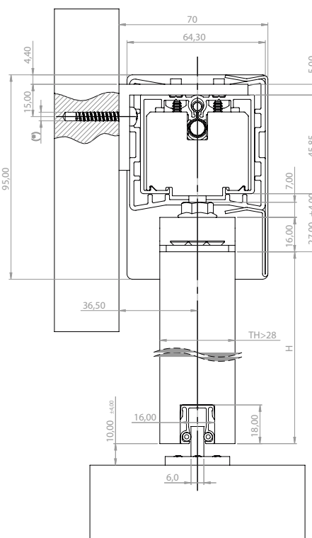
Wall fixing with cover profile
