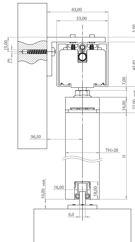
Wall fixing
