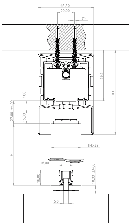
Ceiling fixing with cover profile
