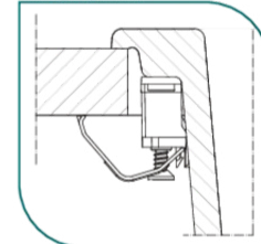
Fixing System
