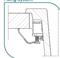
Fixing System
