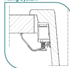
Fixing System
